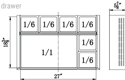
Lower drawer
